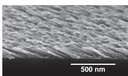
Scanning electron microscope image of a Co F1-STF (tilted 15°) and optical model equivalent
